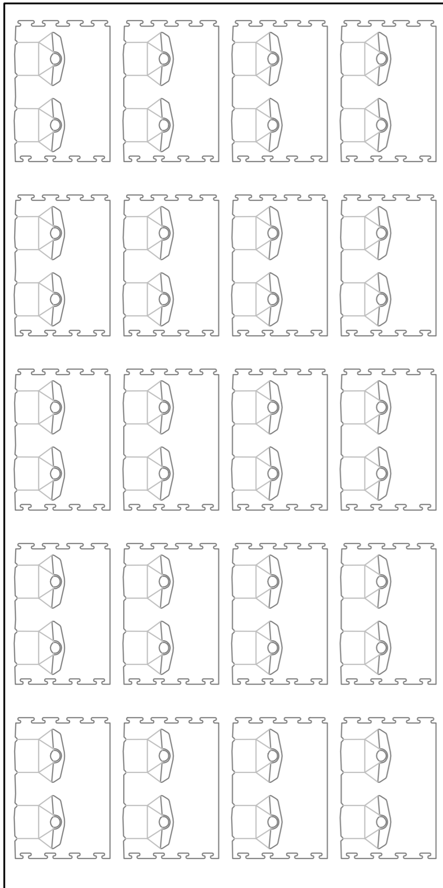
20 Lamps to a 2440 x 1220 Polypropylene Sheet.
